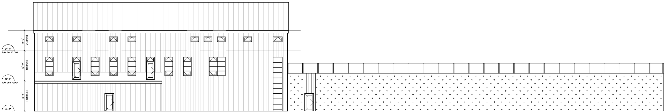
SOUTH ELEVATION
