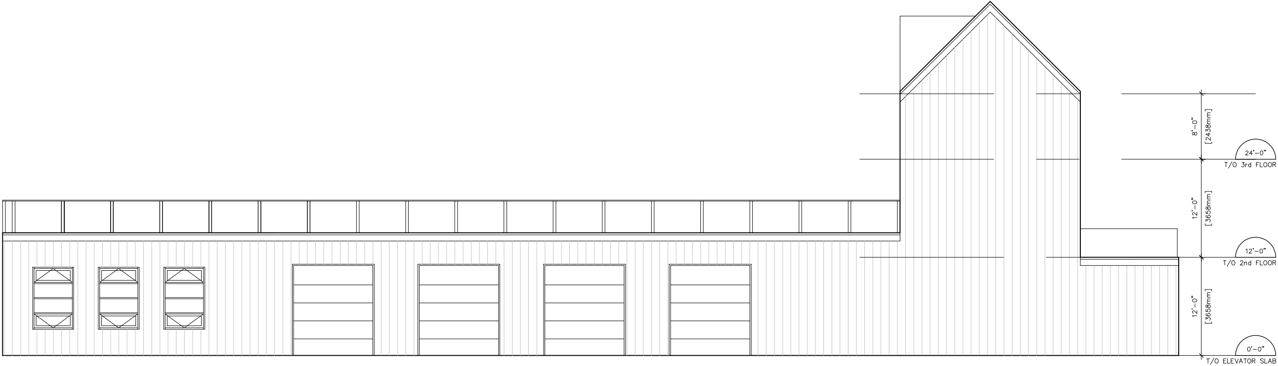
WEST ELEVATION
